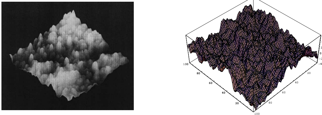
Fig. 1: (a) STM snapshot of a kinetically roughened gold film. The projected area of the sample is 510 \times 510 \text{nm}^2 . Courtesy of Herrasti et al. [5]. (b) Part of a discretized KPZ surface. The entire surface has 400 \times 400 lattice points and is shown after 1000 time steps.
