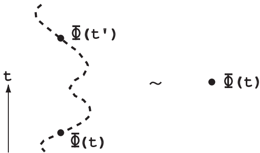
Fig. 4: Operator product expansion of contact fields for a thermally fluctuating string. The short-distance asymptotics of the pair of fields \Phi(t) and \Phi(t') is given by the single field \Phi(t) times a singular prefactor. The dashed line indicates the string configurations generating the singularity |t - t'|^{-x_0} .
