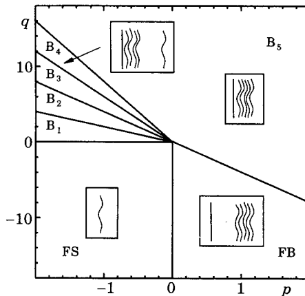
Fig. 2. – Phase diagram for a bundle of N = 5 strings interacting with a wall. The parameter p measures the string-string interaction, the parameter q the string-wall interaction. In regime ( B_n ), n strings are bound to the wall with N - n strings diffusing freely. In the free-bundle regime (FB) the bundle is unbound with respect to the wall. The strings are completely unbound in the free-string regime (FS).
