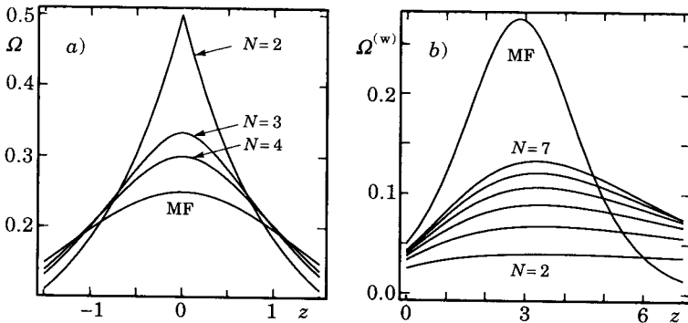
Fig. 1. - a) Density profiles for a free bundle of strings: the exact densities \Omega_N \sim \varphi_N as a function of separation z \sim l for N = 2, 3, 4 strings together with the mean-field density \Omega_{MF} . For increasing N , the exact densities seem to converge towards the mean-field profile. b) Density profile for a string bundle interacting with a wall: the exact densities \Omega_N^{(w)} as a function of separation z \sim l for 2 \leq N \leq 7 together with the mean-field profile \Omega_{MF}^{(w)} for y = -0.95 . The transition from the adhering bundle, regime (B N ), to the free-bundle regime (FB) is located at y_c = -1 .
