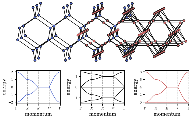
FIG. 18. Diamond-pyrochlore SUSY correspondence. Complex fermions (blue, left) on the diamond lattice are supersymmetrically linked to complex bosons (red, right) on the pyrochlore lattice. The middle panel shows the band structure of the supercharge lattice Hamiltonian on the diamond-X lattice. For the topological classification according to Table II, we find, noting that the Witten index here is \nu = 2 , that the nexus point in the supercharge spectrum has a nontrivial topological invariant of \pi_2 = -1 , see also the illustration in Fig. 25 of the Appendix.
