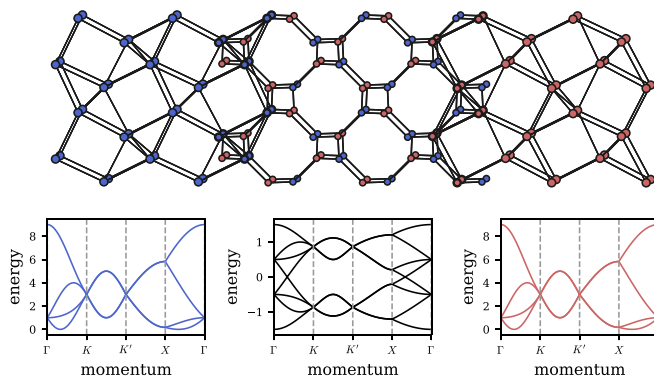
FIG. 16. Spin-fermion SUSY correspondence for the three-dimensional Shastry-Sutherland antiferromagnet. Complex fermions (blue, left) on the hyperoctagon lattice (middle) are supersymmetrically linked to complex bosons (red, right) on a three-dimensional generalization of the Shastry-Sutherland lattice, see Fig. 27 in the Appendix. The ground-state manifold of spin-spiral states for this 3D Shastry-Sutherland model is illustrated in Fig. 17 below. For the topological classification according to Table VI, we find, noting that the Witten index here is \nu = 0 , that the Dirac point between the \Gamma and the K point and that between the X and \Gamma in the supercharge spectrum are topologically trivial (yielding a trivial \pi_1 ).
