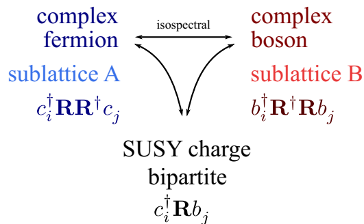
FIG. 5. SUSY matching complex bosons and fermions. Schematic relation between complex bosons and fermions which can be connected by a supercharge defined on a bipartite lattice. In this case, both models are residing on its respective A and B sublattices.
