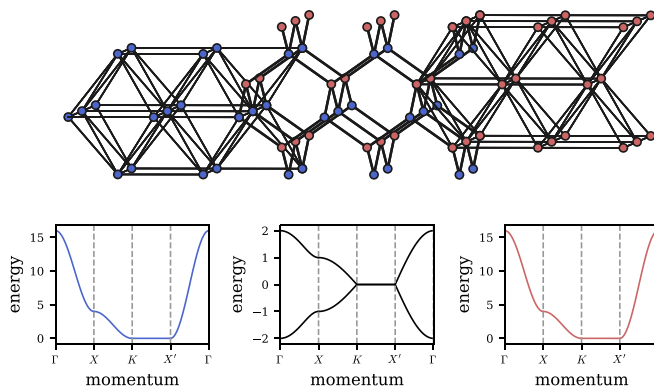
FIG. 15. Spin-fermion SUSY correspondence for the fcc antiferromagnet. Complex fermions (blue, left) on the fcc lattice are supersymmetrically linked to complex bosons (red, right) on the same fcc lattice. The mapping can be established with a supercharge which can be interpreted as the adjacency matrix of a diamond lattice whose two sublattices are the two fcc lattices, respectively. For the topological classification according to Table VI, we find, noting that the Witten index here is \nu = 0 , that the line of Dirac points between the K and K' points in the supercharge spectrum has a nontrivial topological invariant of \pi_1 = +1 (a Berry phase of \pi around the line node).
