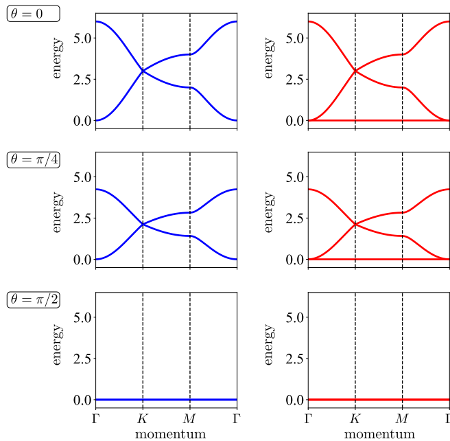
FIG. 7. Kagome lattice magnons (right) and their SUSY partner (left). Spectra are shown along a “ferrimagnetic” path in the XY model ground-state manifold: at the z -polarized ferromagnetic point \theta = 0 (top), at \theta = \pi/4 in the ferrimagnetic region (middle), at the antiferromagnetic q = 0 point \theta = \pi/2 (bottom). These band structures show how ferromagnetic magnons have a quadratic band-touching semimetal as a SUSY partner. Similar to the band structure in Fig. 1, we note that the Witten index is \nu = 1 for all three panels with the quadratic band touching (in the two upper panels) exhibiting a nontrivial \pi_1 topology.
