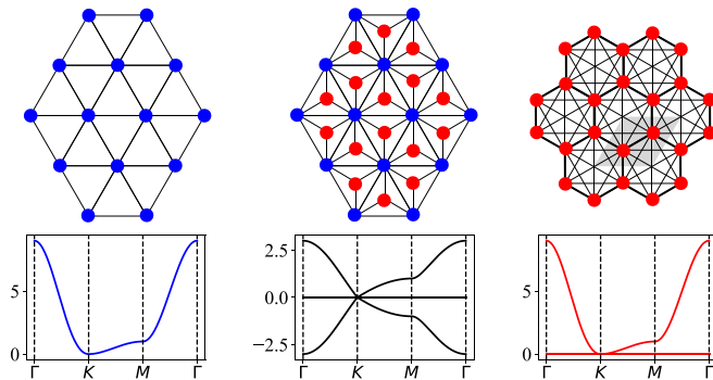
FIG. 4. SUSY beyond the line graph construction. Shown is the SUSY correspondence between complex fermions on a triangular lattice with nearest-neighbor hopping (blue, left) and complex bosons on a honeycomb lattice with further neighbor hoppings (red, right) that falls beyond the line graph lattice construction. For the topological classification according to Table II, we find, noting that the Witten index here is \nu = 1 , that the nexus point in the supercharge spectrum has a nontrivial topological invariant of \pi_1 = +1 .
