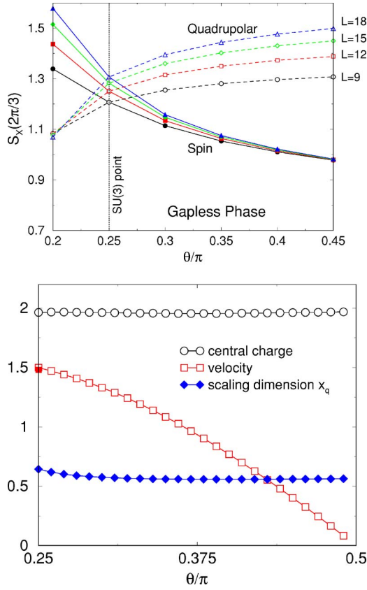
FIG. 2. (Color online) Upper plot: Static structure factors for spin and quadrupolar correlations at momentum k=2\pi/3 as a function of \theta for different system sizes. At the SU(3) point \theta=+\pi/4 the two correlation functions are related by symmetry. By going deeper into the critical region the spin correlations get weaker, while the quadrupolar correlations are enhanced. Lower plot: the central charge, the excitation velocity and the scaling dimension of the quintuplet field in the critical region. The filled red square is the exact result (Ref. 33) for the velocity at \theta=\pi/4 .
