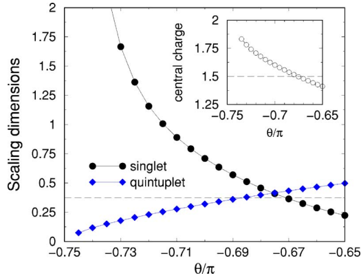
FIG. 8. (Color online) Hypothetical conformal field theory parameters calculated in ED on chains of 8 up to 18 sites. The scaling dimensions of the singlet ( k=\pi ), and the quintuplet ( k=0 ) field are shown. Inset: effective central charge. The value at the boundary of the critical region ( \theta \approx -0.67\pi ) is c \approx 3/2 .
