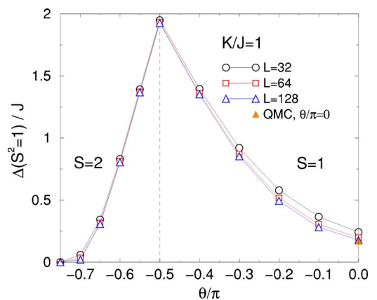
FIG. 11. (Color online) Evolution of the spin gap for constant K/J=1 as a function of \theta \in [-3\pi/4, 0] . The nature of the gap changes at the SU(3) point \theta = -\pi/2 , from a S=1 state for \theta > -\pi/2 to a S=2 state for \theta < -\pi/2 . The QMC value of the gap at \theta=0 is from Ref. 25.
