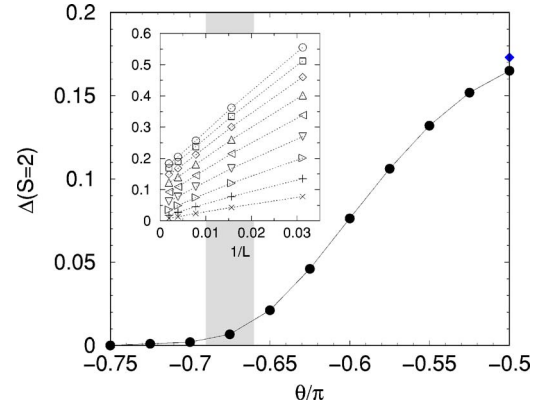
FIG. 3. (Color online) Extrapolated DMRG S=2 gaps as a function of \theta . The gray region denotes the estimated onset of the critical behavior. The filled diamond is the exactly known gap result at \theta=-\pi/2 . Inset: finite size extrapolation of the S=2 gaps (32 to 512 sites). \theta/\pi varies from -0.5 to -0.7 with decrements of 0.025 from top to bottom.
