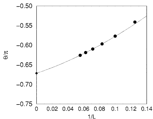
FIG. 5. Finite size scaling of the crossing points between the singlet gap at momentum \pi and the quintuplet ( S=2 ) gap at momentum 0. The extrapolation yields a critical value \theta_c \approx -0.67\pi in the thermodynamic limit.
