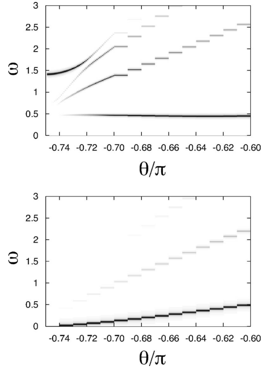
FIG. 7. ED dynamical correlation results on a L=16 chain. Upper panel: dynamical staggered dimer correlation function \mathcal{D}(q=\pi, \omega) plotted for a range of values of \theta . There is an important transfer of spectral weight upon lowering \theta from a low energy level—collapsing to the ground state as a function of system size—to a level which will converge to the energy \sqrt{2} at \theta = -3\pi/4 . Lower panel: dynamical ferroquadrupolar correlations \mathcal{Q}(q=0, \omega) for \theta \in (0.75, 0.60]\pi .
