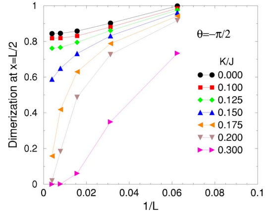
FIG. 10. (Color online) Finite size scaling of the dimerization measured in the middle of a ladder as a function of K/J . It can be clearly seen that the dimerization extrapolates to a finite value for K/J \leq 0.125 , while it tends to zero for K/J \geq 0.15 .
