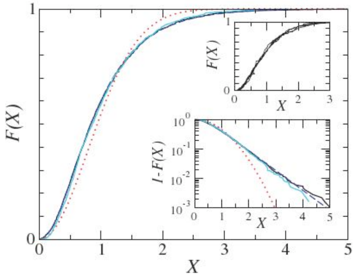
cumulative distribution F(X) : data from real tournaments dashed line = analytical solution for q=0
