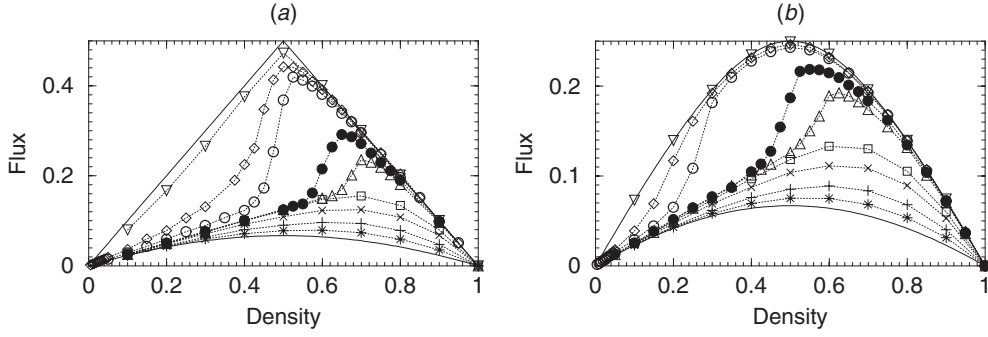
Figure 2. The flux of ants plotted against their densities for the parameters (a) Q = 1 , q = 0.25 and (b) Q = 0.75 , q = 0.25 . The discrete data points corresponding to f = 0.0001(\nabla) , 0.0005(\diamond) , 0.001(\circ) , 0.005(\bullet) , 0.01(\triangle) , 0.05(\square) , 0.10(\times) , 0.25(+) , 0.50(*) have been obtained from computer simulations; the dotted lines connecting these data points merely serve as a guide to the eye. The two continuous curves at the top and bottom correspond to the flux in the NS model for q_{NS} = 1.0 and q_{NS} = 0.25 , respectively, in (a) and for q_{NS} = 0.75 and q_{NS} = 0.25 , respectively, in (b).
