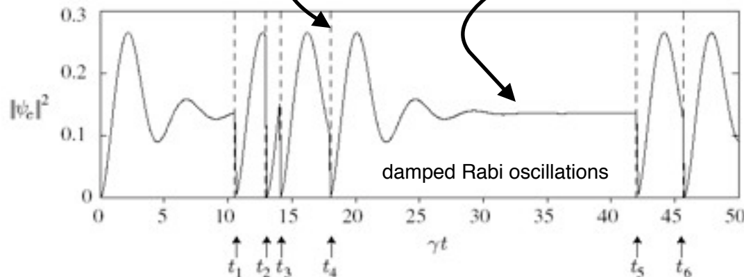
time evolution of upper state population of driven dissipative two-level system (single run)
