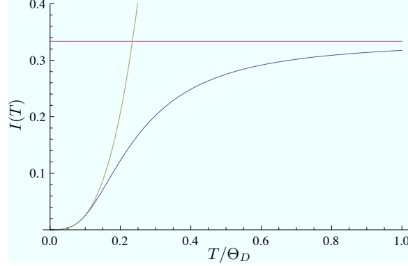
Figure C.1: The shown curves are proportional to \chi_p/T and the low and high temperature approximations to it, respectively.
