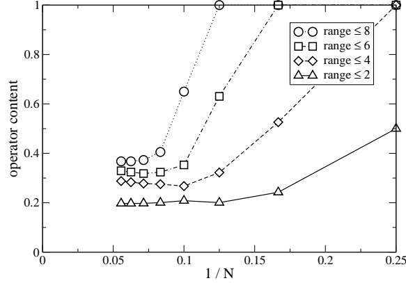
Figure 3.7: Relative weight \sum_{m=1}^n c_m , see Eq. (??), of local operators with range up to n ( n = 2, 4, 6, 8 ) contributing to J_{\parallel} as a function of inverse system size from N = 4 to N = 18 .
