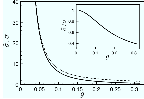
Figure 2.1: Comparison of the result of a single mode memory matrix calculation (solid line), Eq. (??), to the full numerical solution of the Boltzmann equation (dotted line) for T = 0.05 and N = 500 . The memory matrix is always a lower bound to the Boltzmann result and converges towards it as the disorder strength g is reduced, as shown in the inset (ratio of the single mode approximation to the Boltzmann result).
