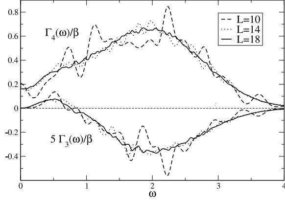
Figure 3.2: Third and fourth order contributions to the scattering rate for various system sizes (see Fig. ??), the first non-vanishing contribution being of order g^4 . Note that finite-size effects are small.
