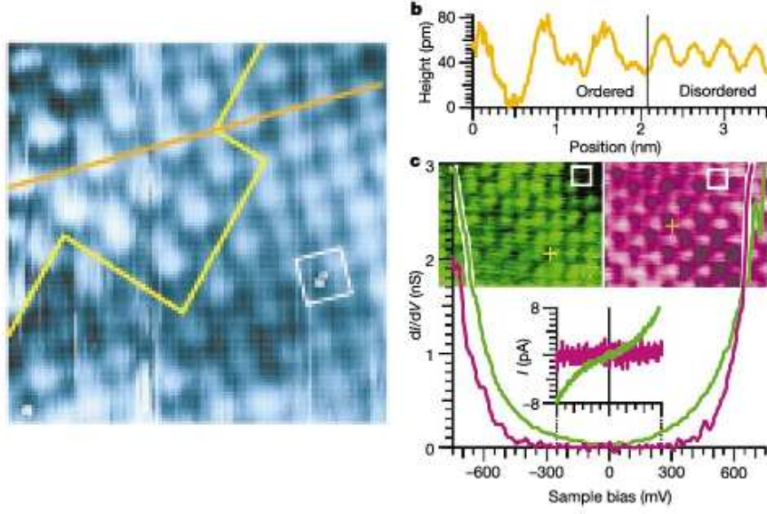
Figure 4.6: Tunneling microscope measurements of the paramagnetic phase of \text{Bi}_{0.24}\text{Ca}_{0.76}\text{MnO}_3 at 299\text{K} . The experiments show a microphase separation of metallic and insulating domains (left panel) with different dI/dV characteristics (right panel). Picture taken from [70].
