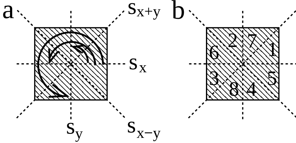
Figure 5.3: Symmetry group of the two-dimensional cubic lattice. Part a: the group contains eight symmetry operations; the identity e , three rotations, R_{\pi/4} , R_{\pi/2} , R_{3\pi/4} , by \pi/4 , \pi/2 and 3\pi/4 , respectively, and four reflections, S_x , S_y , S_{x+y} and S_{x-y} . Part b: the lattice consists of eight identical wedges. If the group elements are put into the order \{e, R_{\pi/4}, R_{\pi/2}, R_{3\pi/4}, S_x, S_y, S_{x+y}, S_{x-y}\} and one arbitrary wedge is identified as wedge "one", one can number the wedges according to the order of the group elements acting on wedge one.
