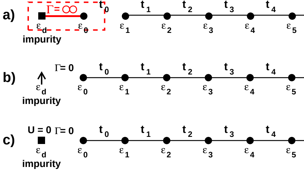
Figure 2.12: (a): Strong-coupling limit, where the effective hybridization \Gamma between the impurity and the first site is so strong that they are decoupled from the chain. The impurity and the first site build a singlet, the Kondo singlet, where the spin of the impurity is screened by the conduction electrons. (b): Local-moment limit, where the impurity is decoupled from the chain and is occupied by one electron due to the interaction U . Thus the degrees of freedom of the impurity are represented by a spin. (c): Free-orbital limit, where the impurity is decoupled and non-interacting. It thus have the four degrees of freedom of a free orbital.
