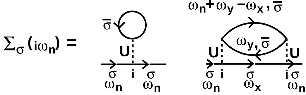
Figure 2.8: Contribution to the impurity self-energy in the iterated perturbation theory (IPT) approximation.
