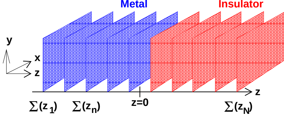
Figure 3.1: Heterostructure of a metallic ( z < 0 ) and insulating ( z > 0 ) system. The system is translational invariant along the layers in x - and y -direction. Thus each site in a layer has the same self-energy, which depends only on the z -coordinate.
