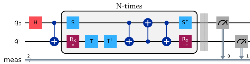
Figure 4 – Circuit 2 (long).
