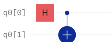
Figure 2 – Bell state circuit.
