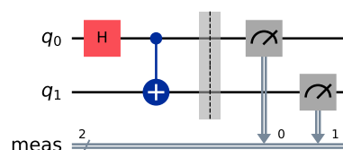
Figure 3 – Circuit 1 (short).
