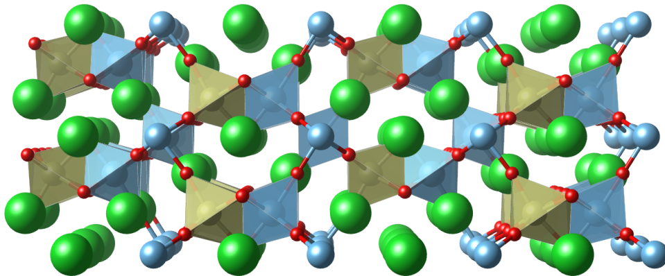
Figure 1: \text{Ba}_3\text{IrTi}_2\text{O}_9 .
