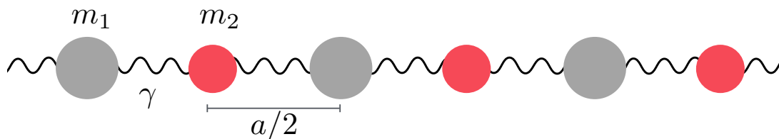
Figure 1: A diatomic chain with two types of atom of masses m_1 and m_2 that are connected by a spring with constant \gamma . At rest each atom is separated from its neighbor by a distance a/2 . Oscillations only occur along the chain and not perpendicular to it i.e. we consider only acoustic modes.
