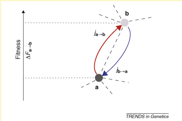
Figure I. Equilibrium state under time-independent selection.
